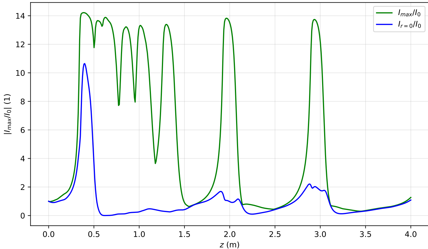
I_{max}(x=0, y=0, z)/I_0 , P_{in}=7.8P_{cr} , noisy input, artificial time
